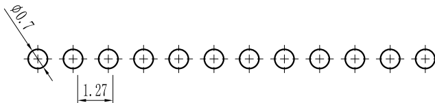
PCB LAYOUT
