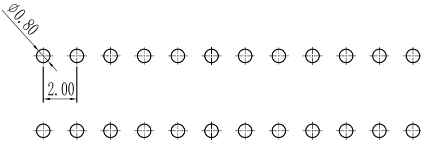
PCB LAYOUT
