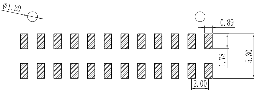
PCB LAYOUT
