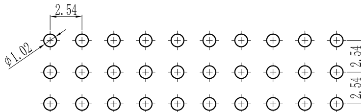
PCB LAYOUT
