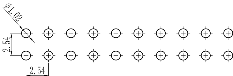
PCB LAYOUT
