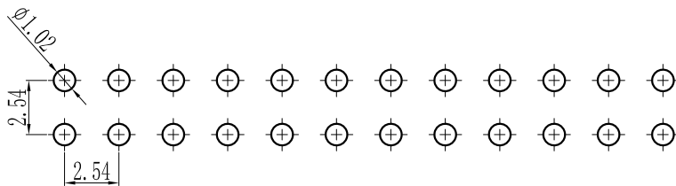
PCB LAYOUT
